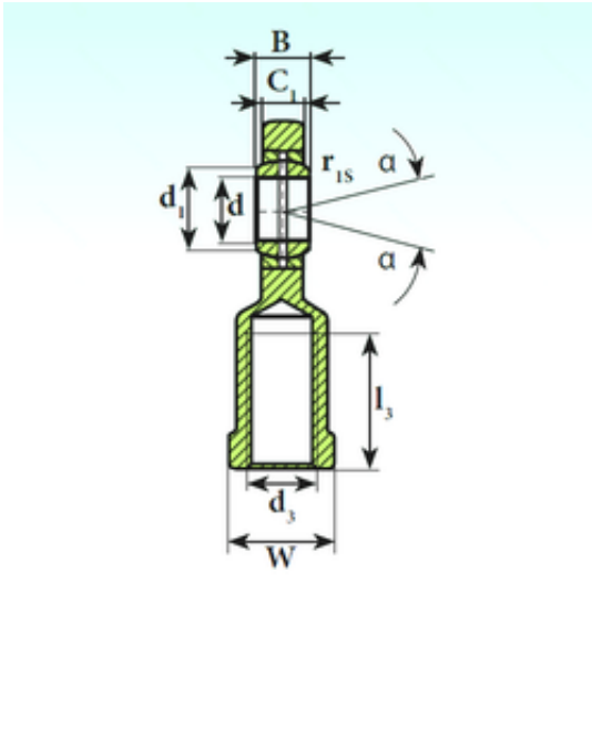
SI 30 ES Bearing 2D drawings and 3D CAD models
